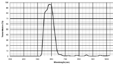
BP635 RED BANDPASS
