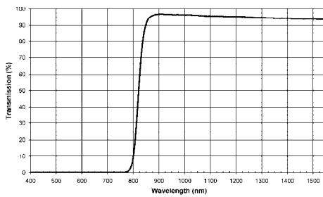
LP830 INFRARED LONGPASS
